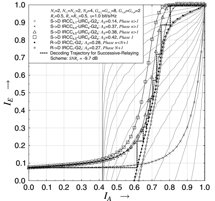
Fig. 7. The EXIT chart curves for the IRCC s -URC s -G 2s with various "inner" iterations, the IRCC s -G 2s with IRCC s having optimized weighting coefficients [\beta_1, \dots, \beta_{17}] = [0, 0, 0, 0, 0.233115, 0.0158742, 0.292084, 0.220065, 0.0151108, 0, 0, 0, 0, 0, 0, 0.22375] and 17 SNR-dependent IRCC r -G 2r subcodes. The subscript of IRCC s denotes the number of "inner" iterations between the IRCC s and "G 2s -URC s " decoders and the \text{SNR}_e^r represents the equivalent SNR at the source and relays.
