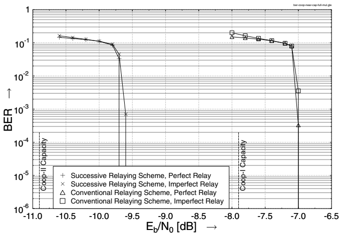
Fig. 8. BER versus E_b/N_0 performance of both perfect and imperfect relaying aided Ir-DST coding schemes in the successive relaying aided network for a frame length of 250 000 bits, while the performance of the single-relay-aided scheme in [10] is also depicted here for comparison.
