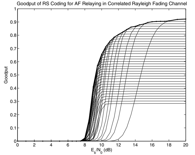
Fig. 6. Effect of code rate on the achievable goodput in ReS coded H-ARQ using AF relaying where we have k/n = 0.3 \div 0.98 in steps of 0.02, the remaining parameters provided in Table I.
