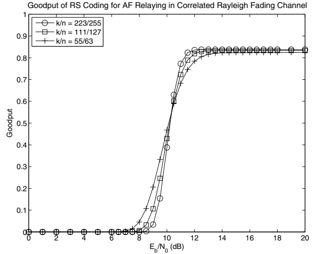
Fig. 5. Effect of codeword length on the achievable goodput in ReS coded H-ARQ using AF relaying where we have k/n = \{223/255, 111/127, 55/63\} , the remaining parameters are provided in Table I.
