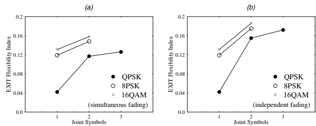
Figure 6: EXIT flexibility index F_I , when considering various number of joint symbols and different modulation schemes. (a) The case of a simultaneous fading based Rayleigh channel model. (b) The case of an independent fading based Rayleigh channel model.
