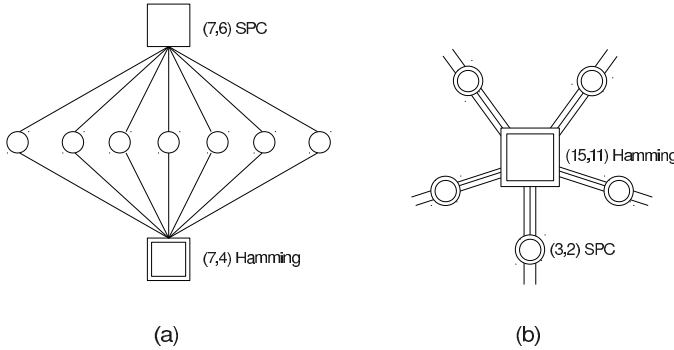
Fig. 1. (a): R = 3/7 GLDPC protograph. All VNs are repetition-2 codes, one CN is a (7, 4) Hamming code and the other a (7, 6) SPC code. (b): R = 3/5 D-GLDPC protograph. All VNs are (3, 2) SPC codes and the CN is a (15, 11) Hamming code.
