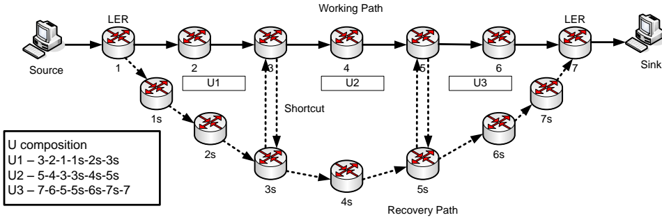
Figure 5: Example of resulting U chain.
