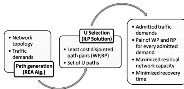
Figure 6: Scheme of the network engineering algorithm.
