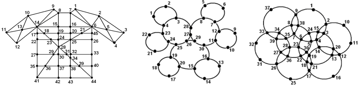
Figure 7: Investigated topologies (from left to right): Mesh, Molecule and Maze.
