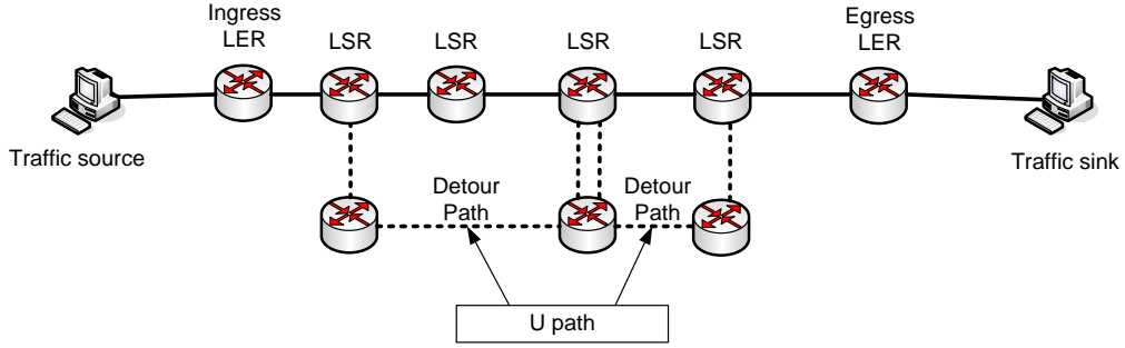
Figure 3: U-path examples
