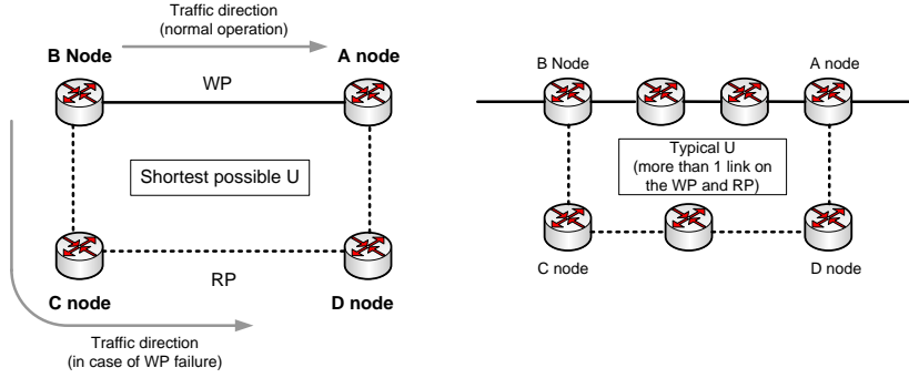
Figure 4: U-path decomposition.
