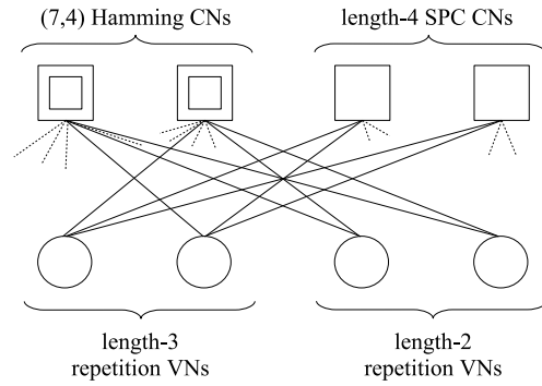
Fig. 1. Example of valid assignment of weight 10. The solid edges belong to the assignments, the dashed edges do not belong to it.
